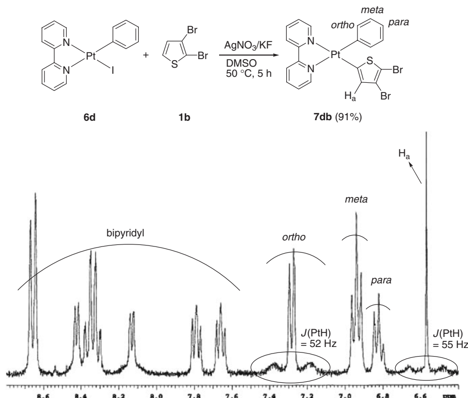
Figure 1. Synthesis of platinum(II) complex 7db and its ^1\text{H} NMR spectrum of platinum(II) complex 7db (300 MHz, \text{DMSO}-d_6 , rt).
