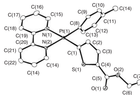
Figure 2. ORTEP drawing of 7ee (50% probability). Hydrogen atoms were omitted for clarity.
